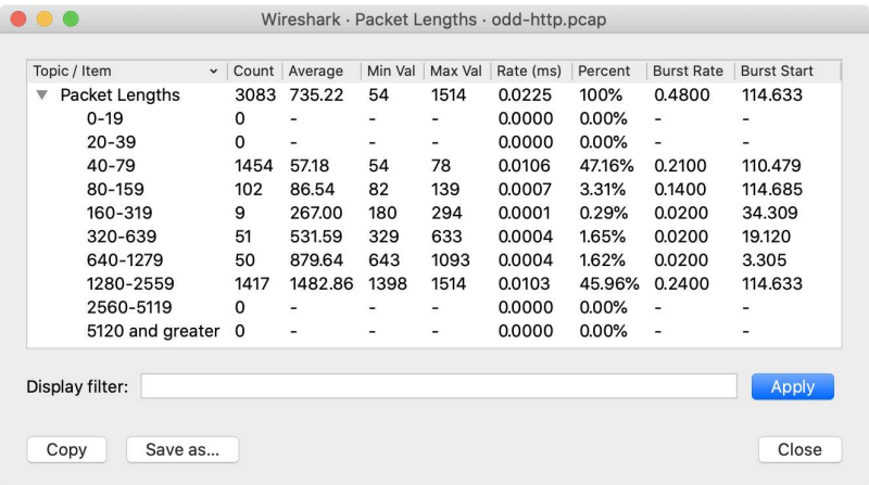
Figure 83. The “Packet Lengths” window
