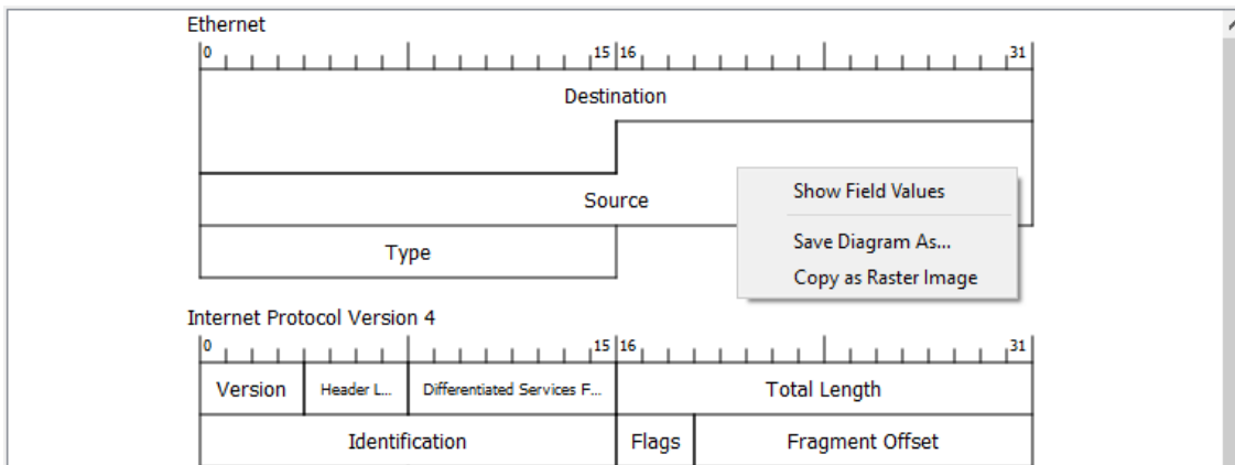
Figure 60. Pop-up menu of the “Packet Diagram” pane
